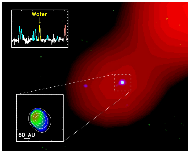
Figure 2: Radio image obtained with the IRAM interferometer: Top left the spectral “fingerprint” of water can be clearly discerned. Bottom left, the distribution of water in the disk around the young star NGC 1333 IRAS4B is shown.
